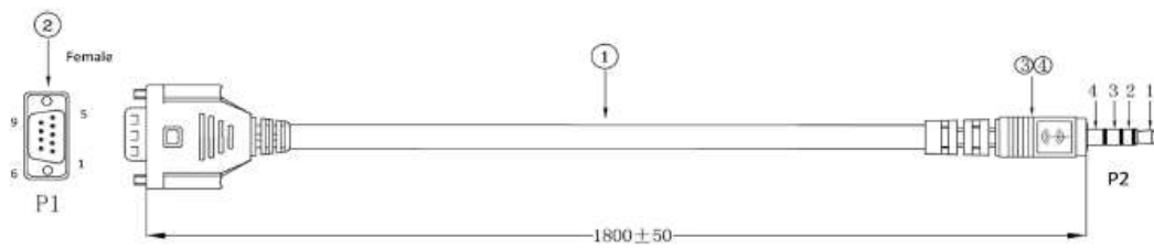
Female D-Sub 9-Pin (outside view)
